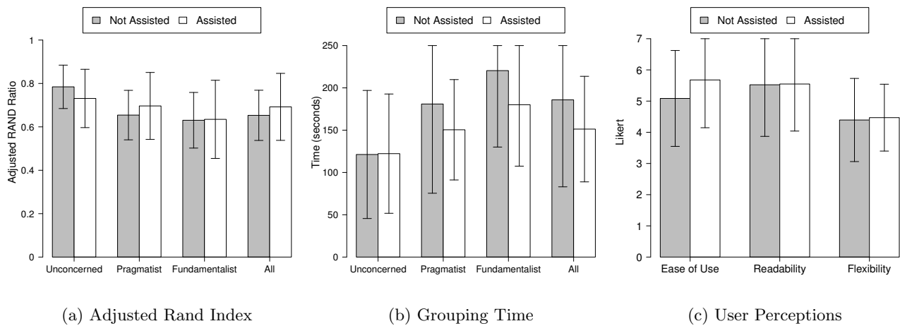
Figure 7: Not Assisted vs. Assisted Friend Grouping
