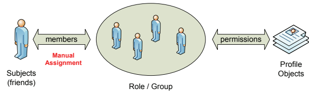
Figure 1: Role Based Access Control
